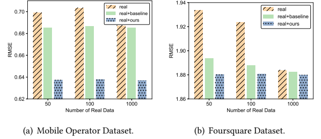
Figure 12: Interval estimation with data augmentation. For a different number of real-world sequences, i.e. , 50, 100, 1000, we all add 1000 generated sequences for data augmentation.
